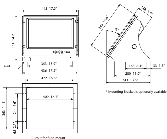
MU-170C 12.9 kg 28.4 lb
