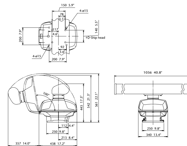
3.5' Open Radar Sensor DRS4A 25 kg 55.1 lb
